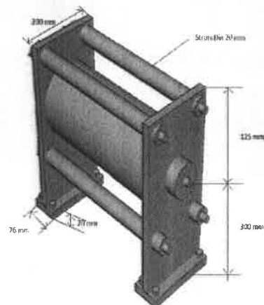
Fig. 4 Schematic of Pneumatic Gas Gun
