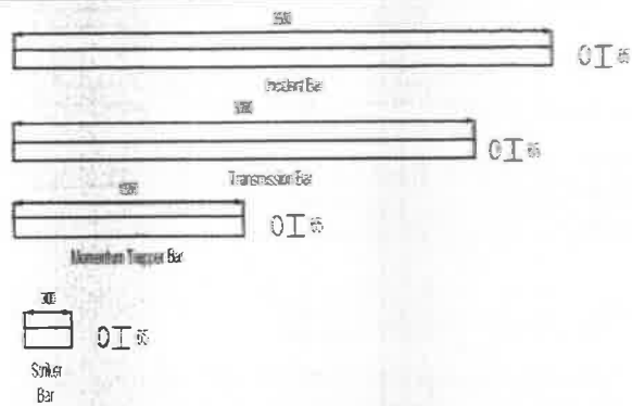
Fig. 2 Details of Steel Bars (All dimensions in mm)
