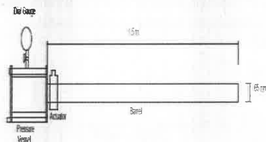
Fig. 4 Schematic of Pneumatic Gas Gun
