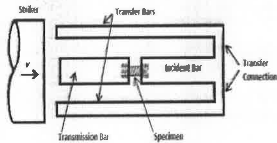
Fig. 3 Direct acting tension loading for metal testing
